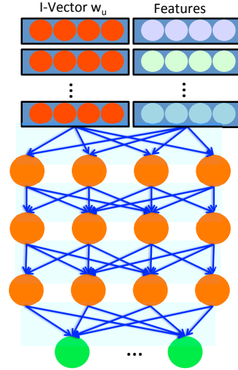
Figure 2: Using i-vector as a speaker feature vector
